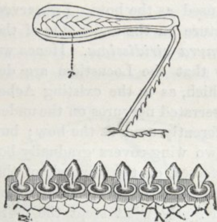
FIG. 13.—Hind-leg of Stenobothrus pratorum : r , the stridulating ridge; lower figure, the teeth, forming the ridge, much magnified (from Landois).
